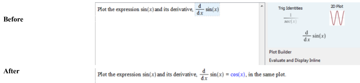
Figure 7.10: Working with Document Blocks
