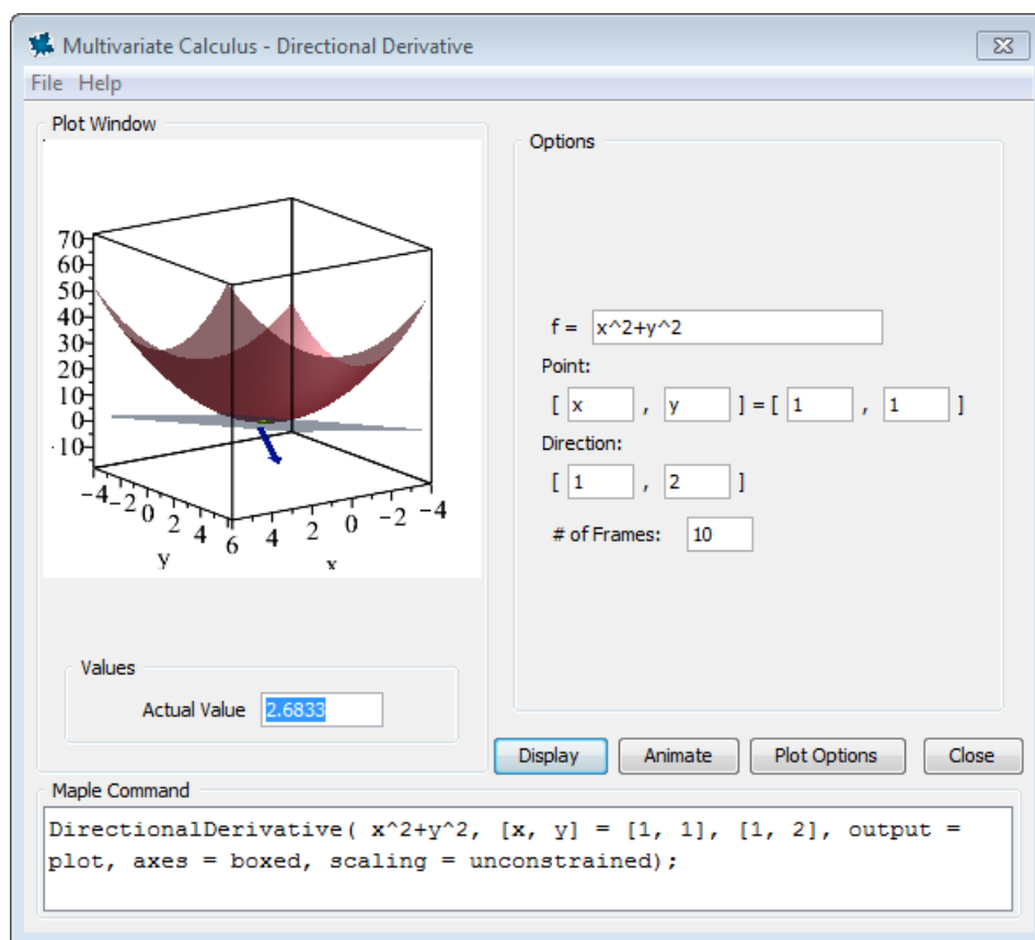
Figure 5.7: Directional Derivative Tutor
