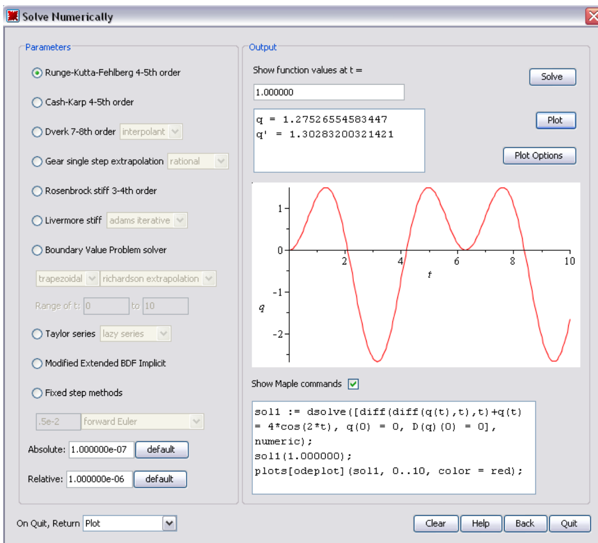
Figure 4.4: ODE Analyzer Assistant: Solve Numerically Dialog
