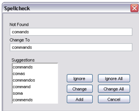
Figure 7.23: Spellcheck Dialog
