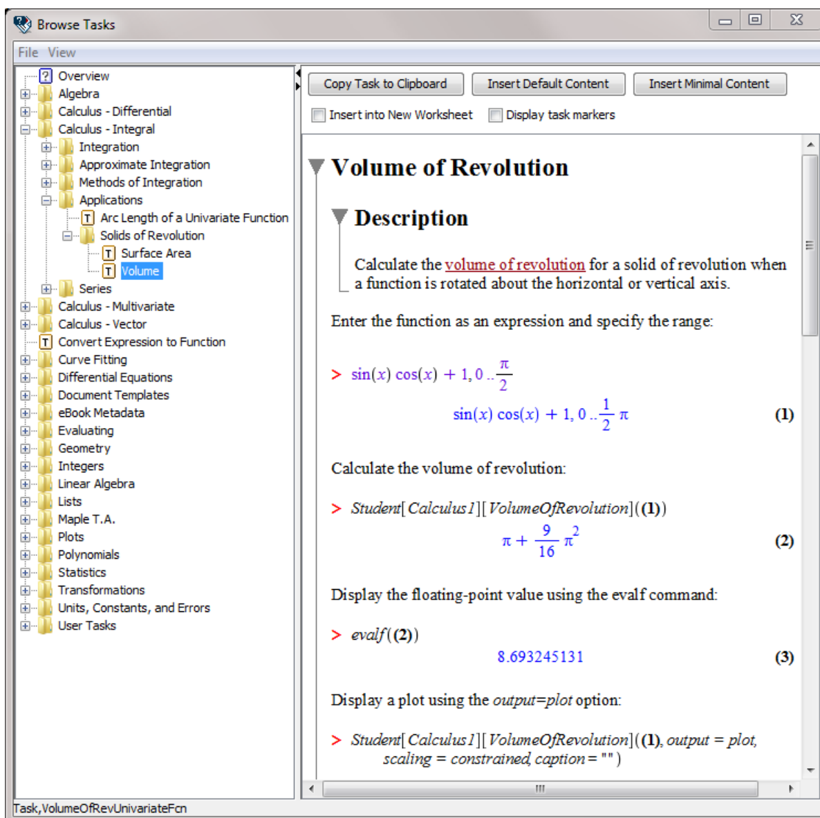
Figure 3.4: Task Browser
