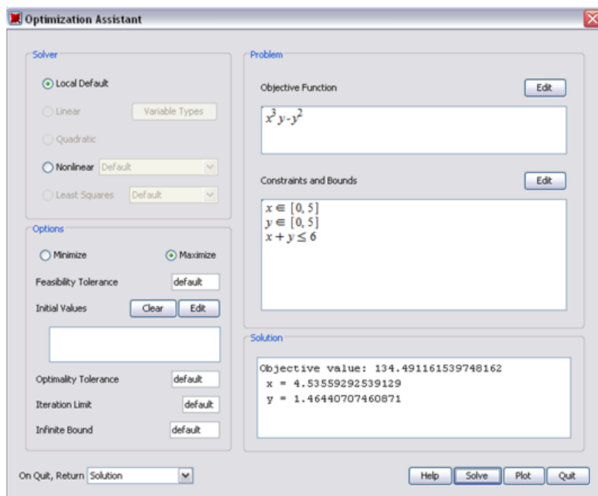
Figure 5.8: Optimization Assistant
