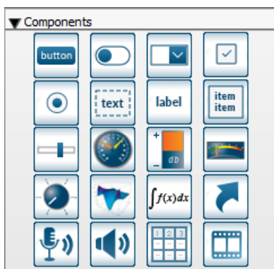
Figure 7.21: Components Palette
