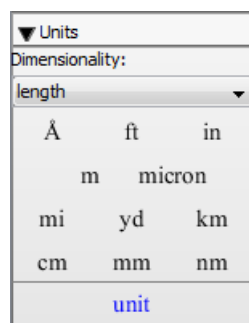
Figure 2.4: Units Palette
