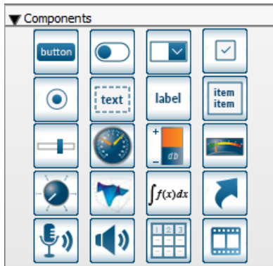
Figure 10.1: Components Palette
