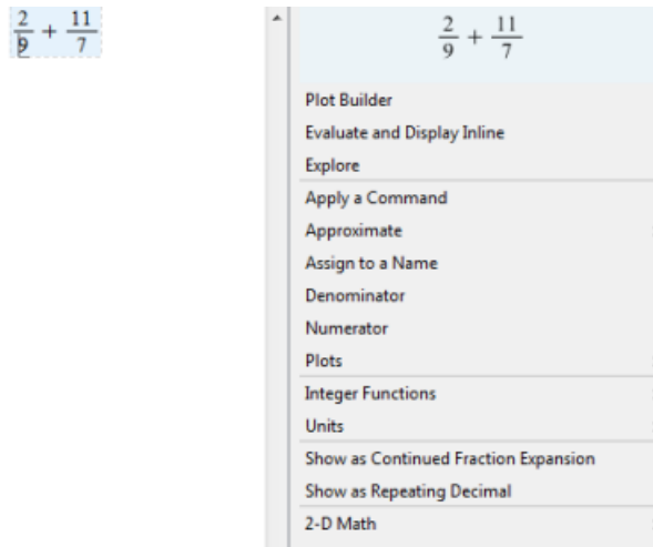
Figure 2.1: Context Panel
