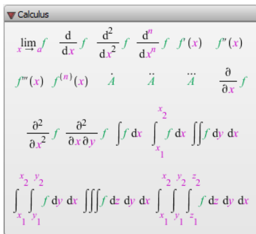
Figure 3.1: Calculus Palette
